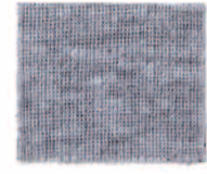
Baby Rib —100% Ring-Spun Combed Cotton —5.8 oz/yd 2 (197 g/m 2 ) —30-singles
